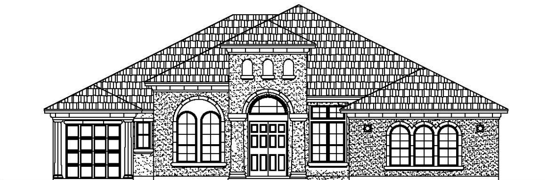
MEDITERRANEAN ELEVATION
